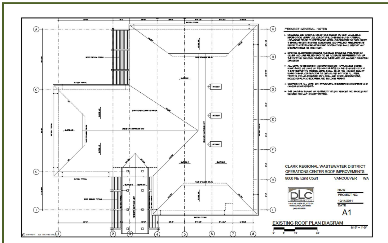
Existing Operations Center Roof Diagram
